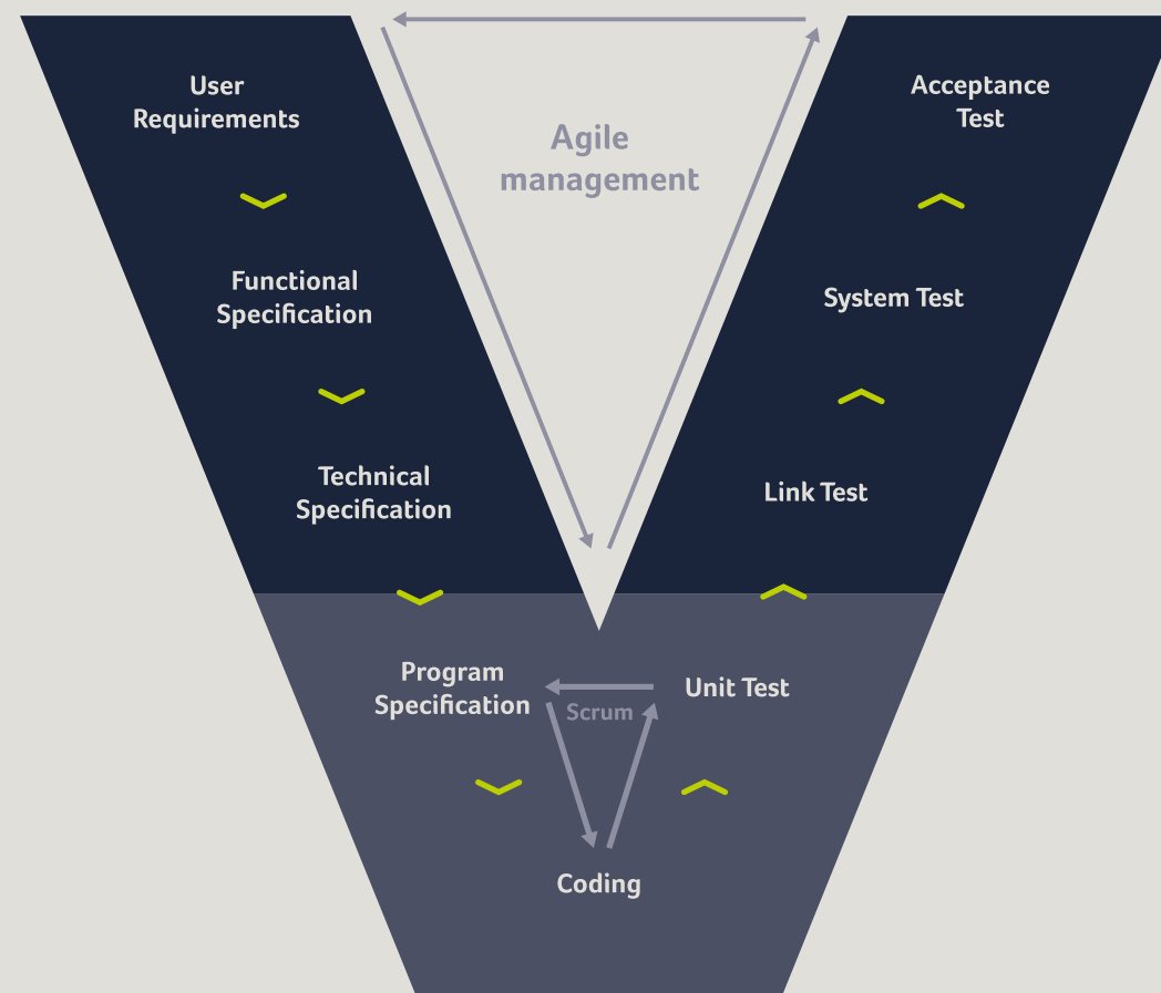
The agile V-model
